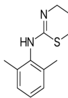
FIGURE 1. Structure of xylazine
