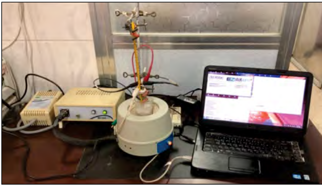
FIGURE 3. Cyclic voltammetry set up
